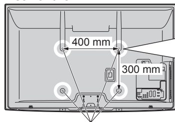
Holes for wall-hanging bracket installation
