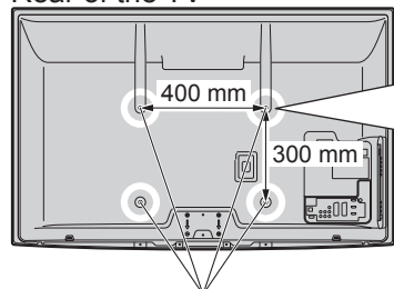
Holes for wall-hanging bracket installation
